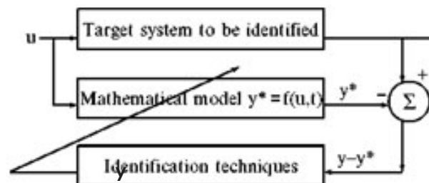
Figure Block Diagram for Parameter Identification
