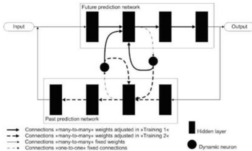
Fig. Bi-directional artificial neural network
