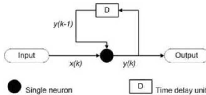
Fig. Simple “one neuron” Hopfield artificial neural network
