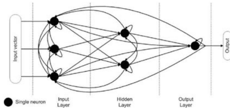
Fig. Fully recurrent artificial neural network
