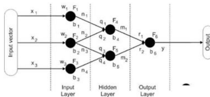
Fig. Feed-forward artificial neural network.
