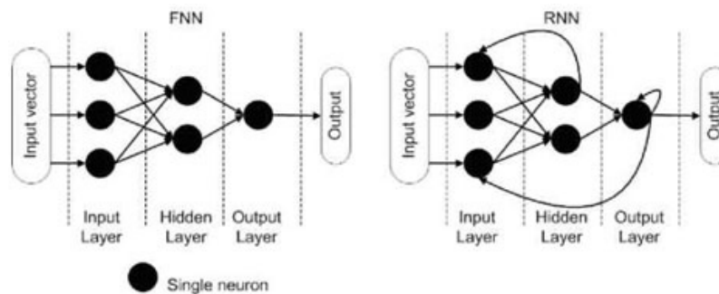
Fig. Feed-forward (FNN) and recurrent (RNN) topology of an artificial
