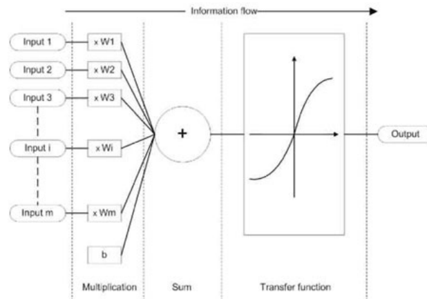
Fig. Working Principle of an Artificial Neuron
