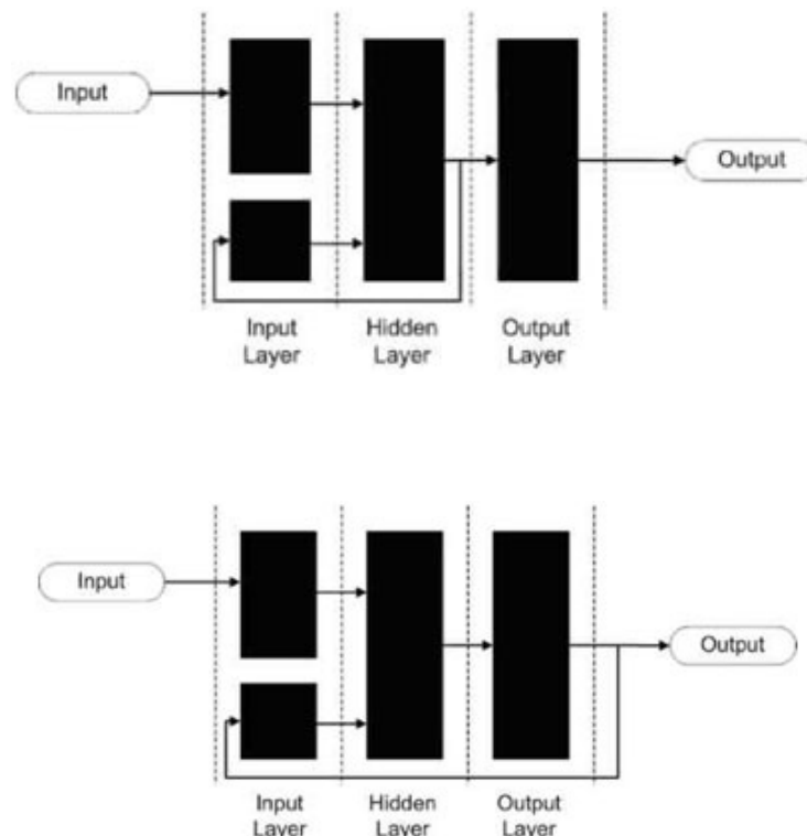
Fig. Jordan artificial neural network
