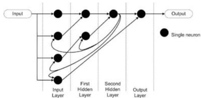
Fig. Simple Long Short Term Memory artificial neural network (block)
