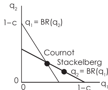
Stackelberg Competition
